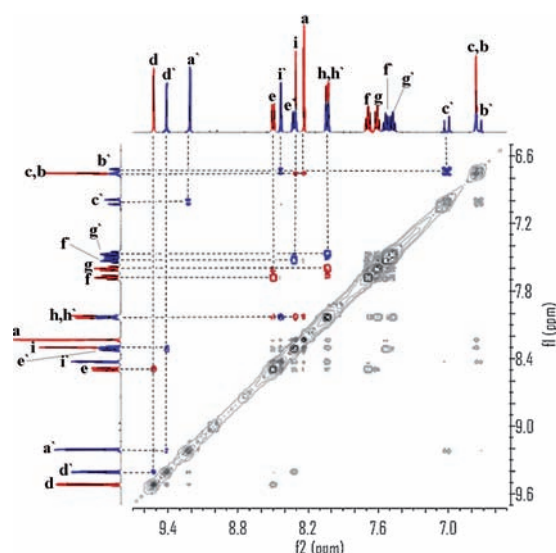
Figure 3. Partial NOESY spectra of complex \mathbf{1b} \cdot 4\text{PF}_6^- in [\text{D}_3]\text{acetonitrile} solution at 298 K.
