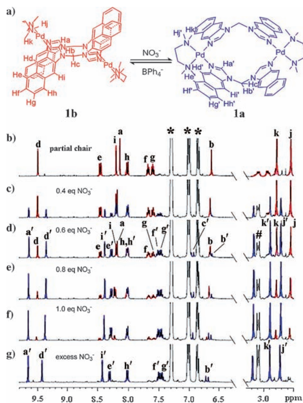
Figure 2. a) The conformation transformation between partial-chair and bowl-shaped structure; and ^1\text{H} NMR spectra (in [\text{D}_3]\text{acetonitrile} at 298 K) of b) complex \mathbf{1b} \cdot 4\text{BPh}_4^- ; after adding c) 0.4 equiv; d) 0.6 equiv; e) 0.8 equiv; f) 1 equiv; g) excess (based on \mathbf{1b} \cdot 4\text{BPh}_4^- ) of [\text{nBu}_4\text{N}]\text{NO}_3 . (Bowl-shaped conformer represented by a'–i'; partial chair conformer represented by a–i; * signals from \text{BPh}_4^- ; # signals from \text{tBu}_4\text{N}^+ ).
